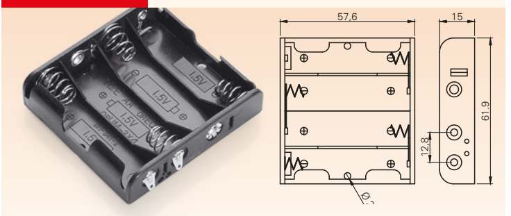
4 PCS AA SIZE BATTERY HOLDER
