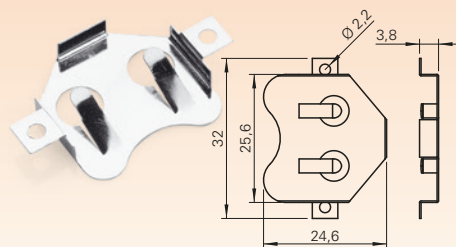
CR-2430 BATTERY HOLDER
