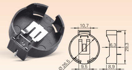
CR-2450 BATTERY HOLDER
