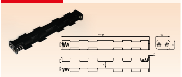
6 PCS AA SIZE BATTERY HOLDER
