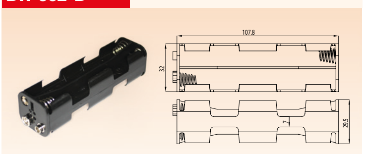
8 PCS AA SIZE BATTERY HOLDER
